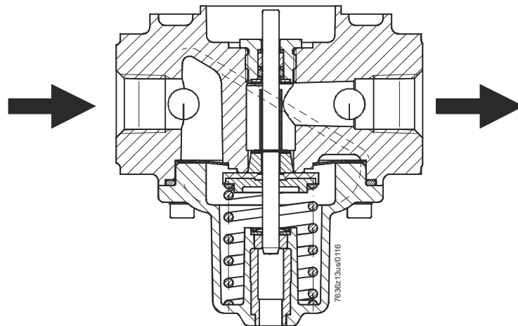
Figure 1. Sectional view of VGG10.xxxU models
