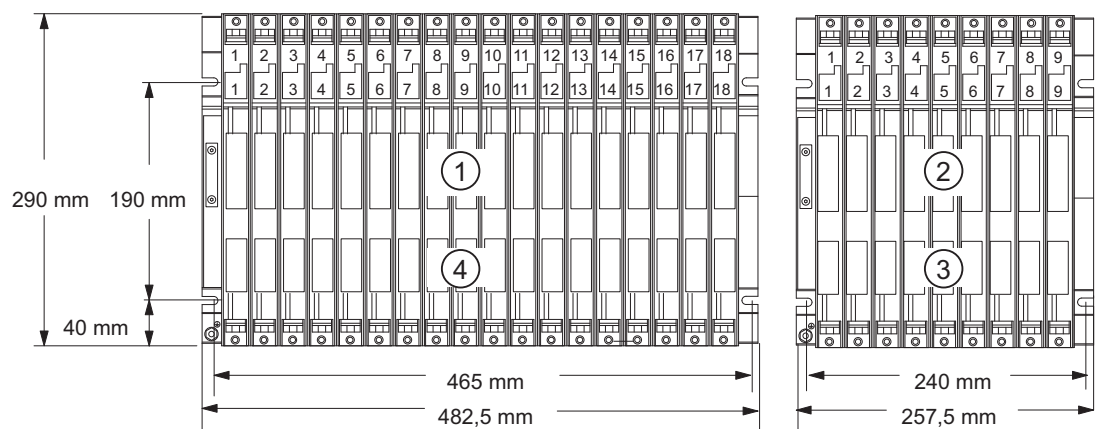
Figure 2-2 UR1 rack with 18 slots and UR2 with 9 slots
