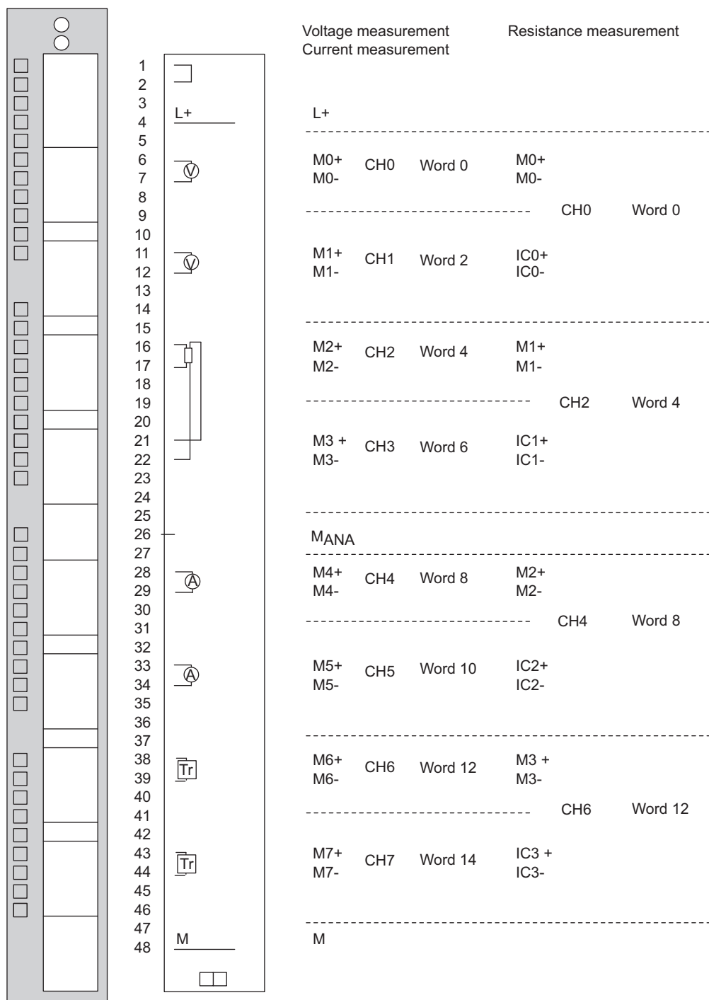
Figure 5-28 Connection diagram for SM 431; AI 8 x 14 bit
