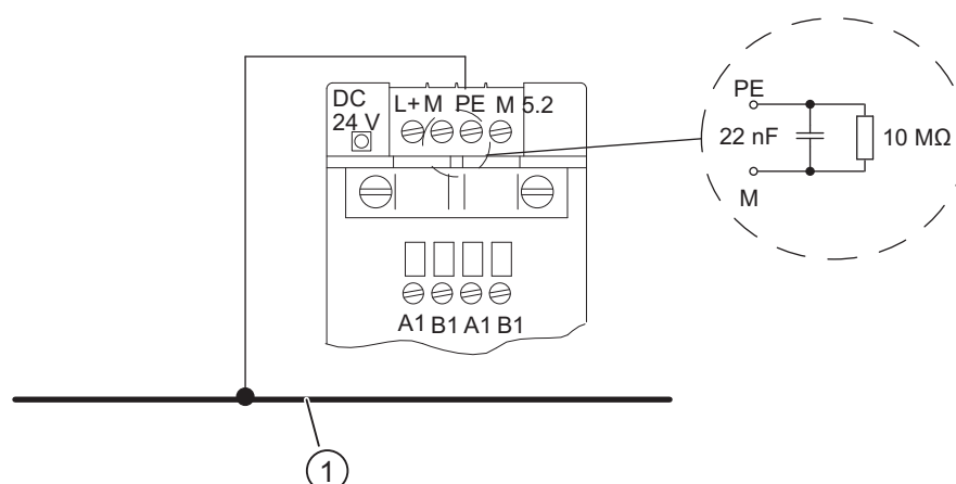
Figure 10-1 RC network with 10 M Ohm for configuration with ungrounded reference potential (1) Ground busbar
