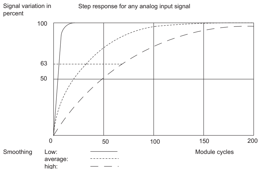
Figure 5-26 Step response of the SM 431; AI 8 x 14 Bit
