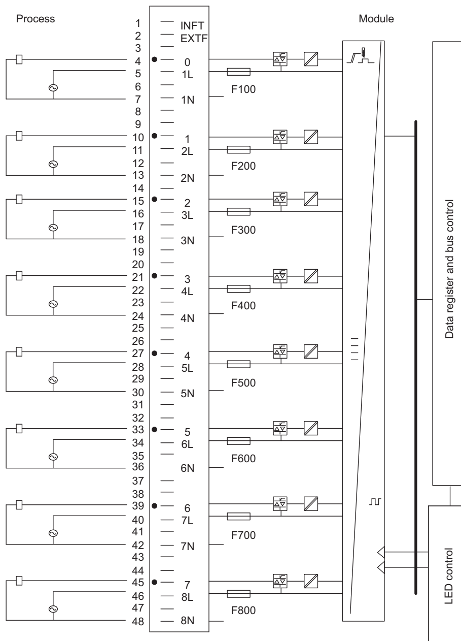
Figure 4-15 Connection and circuit diagram for SM 422; DO 8 x AC 120/230 V/5 A
