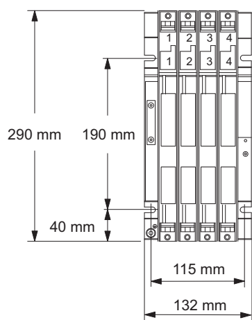
Figure 2-5 CR3 rack
