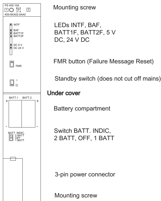
Figure 3-11 PS 405 10A and PS 405 10A R operator control and monitoring elements
