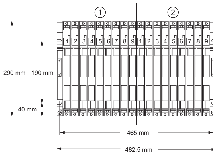
Figure 2-3 Rack dimensions
