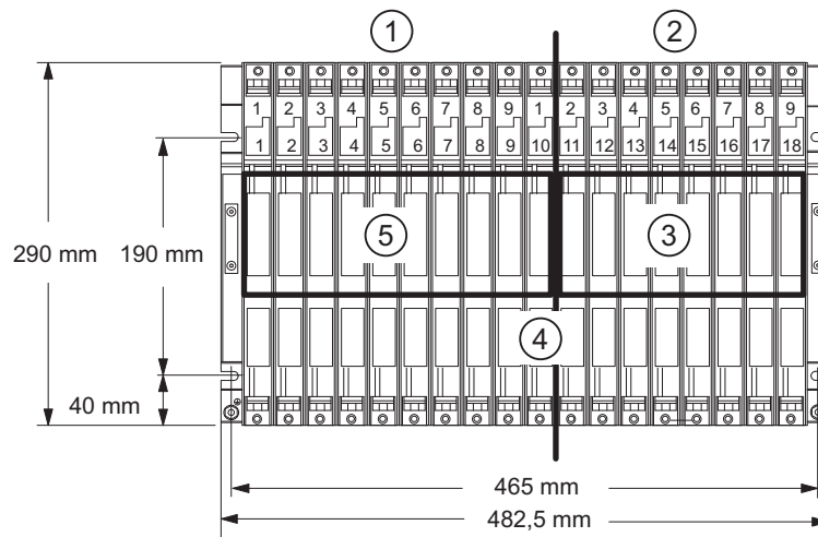
Figure 2-4 CR2 rack
