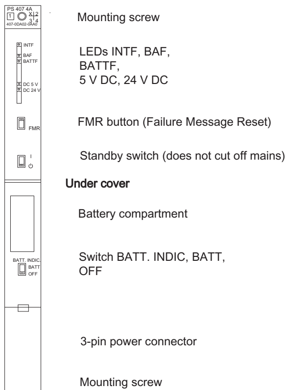
Figure 3-3 PS 407 4A operator control and monitoring elements
