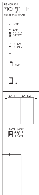
Figure 3-13 PS 405 20A operator control and monitoring elements
