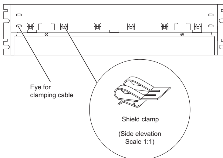
Figure 9-2 Front view of the cable duct
