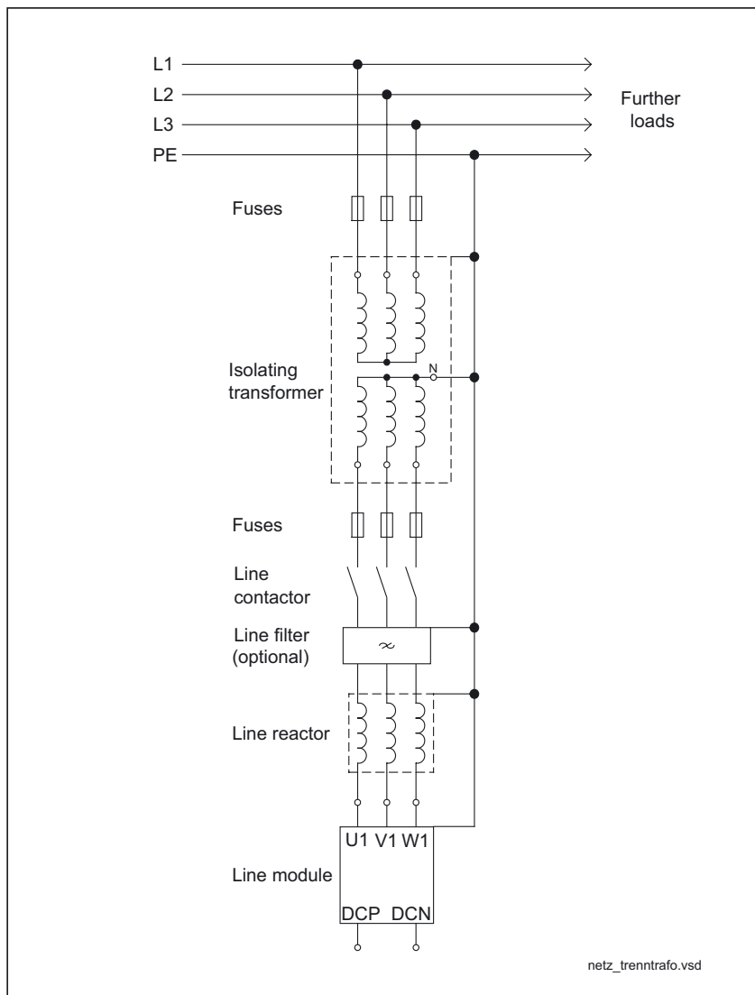
Figure 2-5 Isolating transformer
