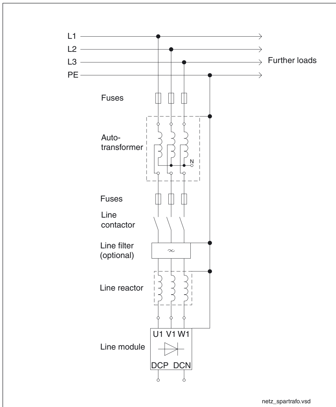
Figure 2-4 Autotransformer
