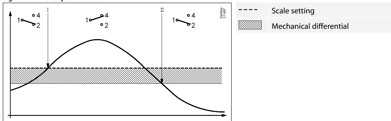
Figure 4: Contact system function
