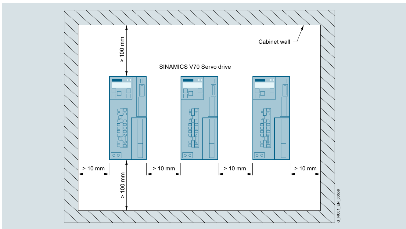
Mounting clearance
