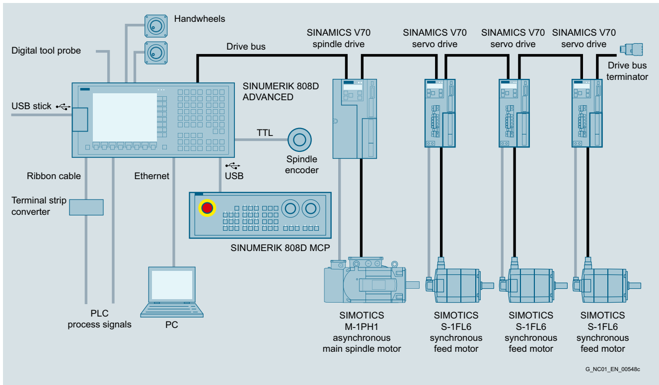
SINUMERIK 808D ADVANCED system
