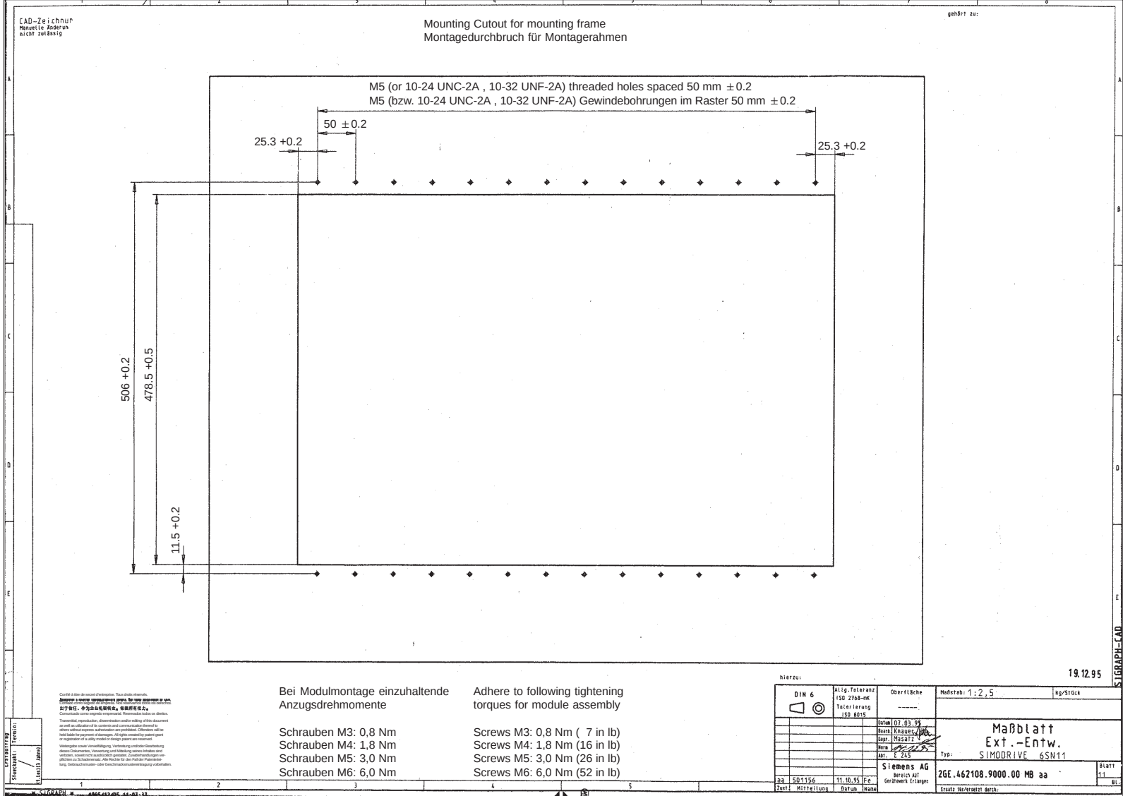
Fig. 12-444 External cooling, installation cutout for installation frames
