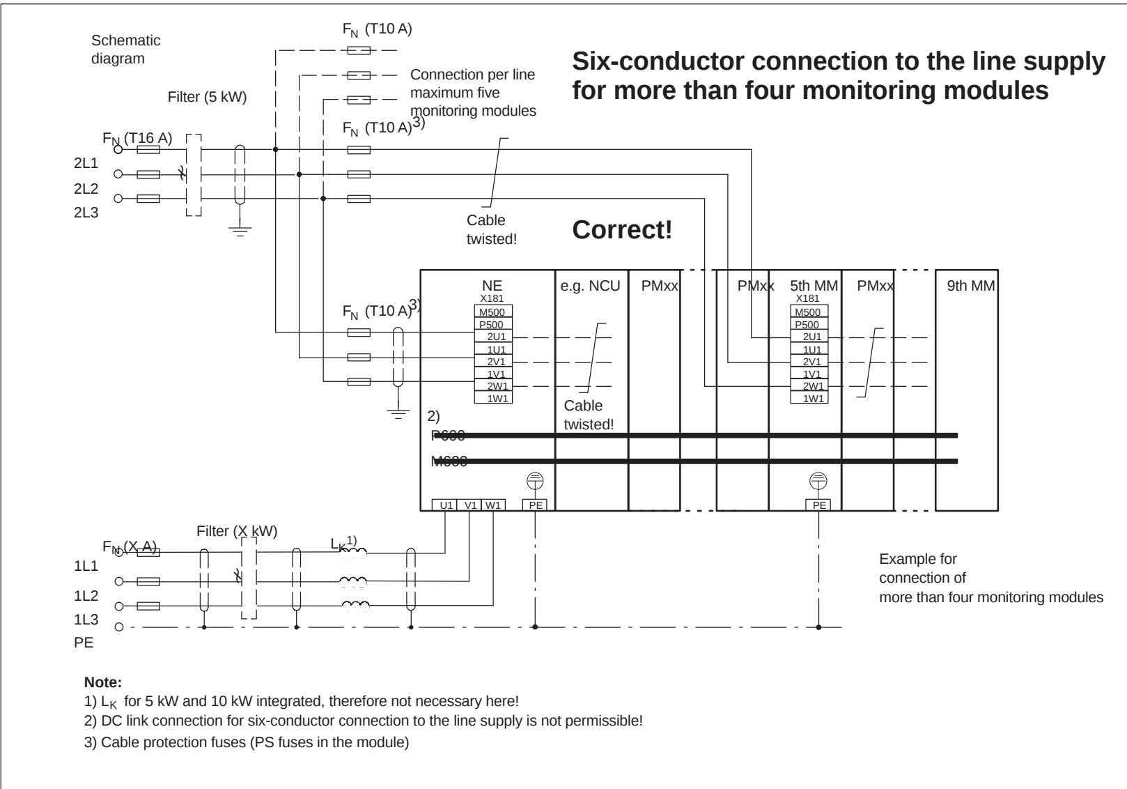
Fig. 8-34 Examples for correct six-conductor connection to the line supply with more than four monitoring modules connected to a line infed module (NE module)
