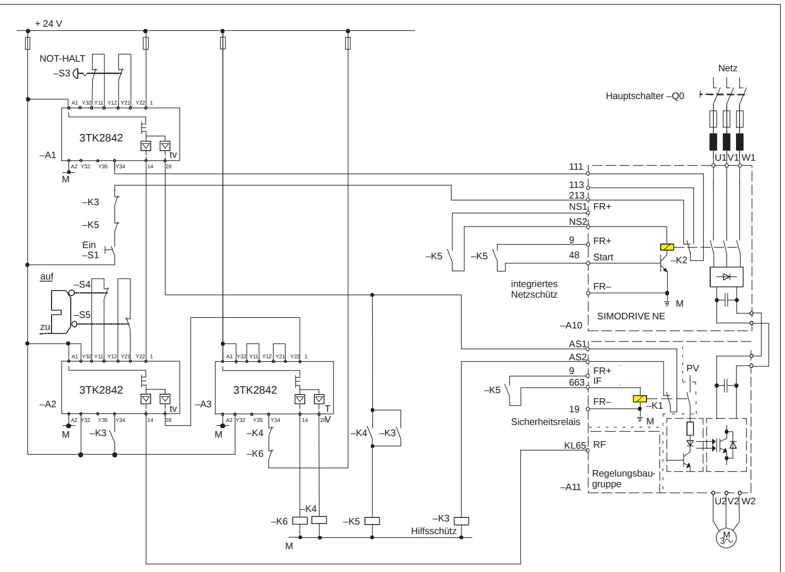
Fig. 9-16 EMERGENCY STOP and protective door monitoring at a SIMODRIVE 611 universal converter – SS1 at the drive
