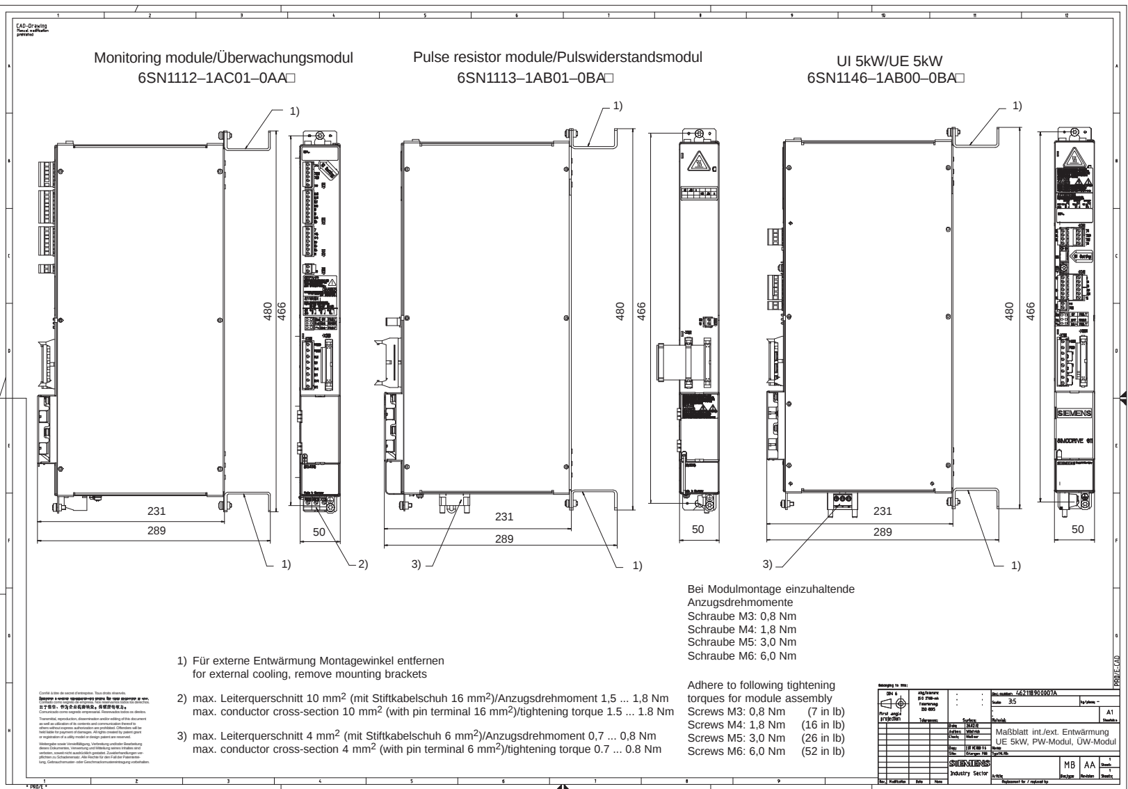
Fig. 12-41 Internal/external cooling, 50 mm UI module (6SN1146-1AB00-0BAx); pulse resistor module (6SN1113-1AB01-0BAx); monitoring module (6SN1112-1AC01-0AAx)
