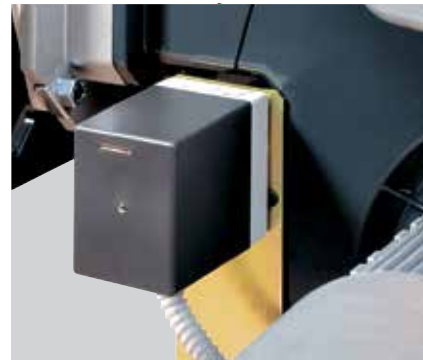
Example of the servomotor for air/oil setting
