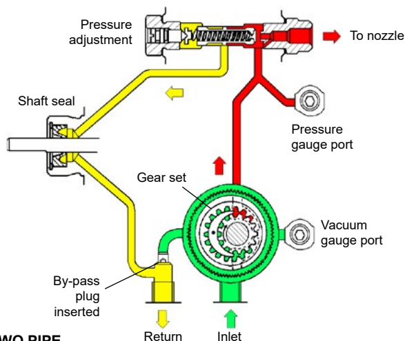
TWO PIPE INSTALLATION
