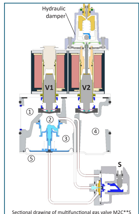
Sectional drawing of multifunctional gas valve M2C**S
