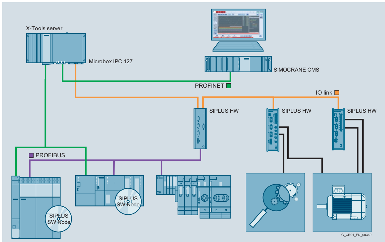
Configuration of using Fast Trace
