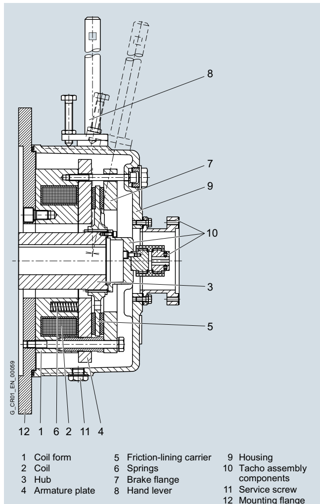
KFB spring-set brake with manual lever
