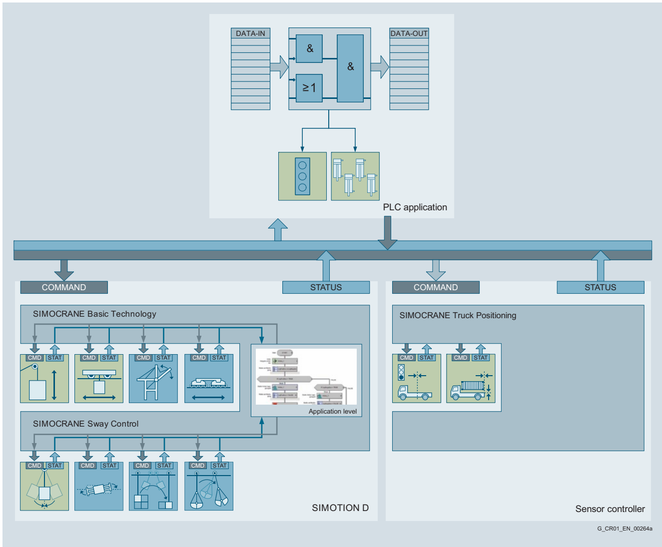
Function blocks of the application example for a semi-automatic STS crane
