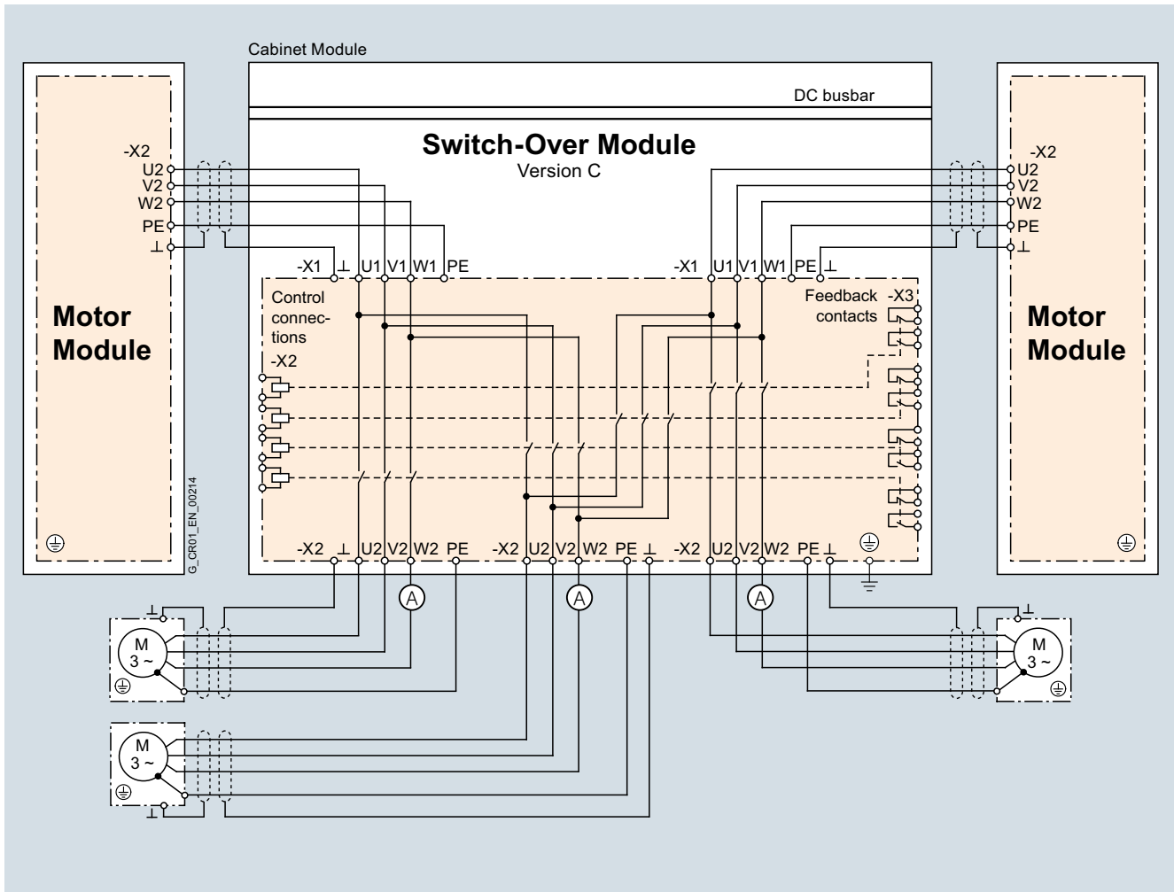
Connection example of a Switch-Over Module, Version C
