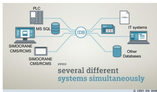
Example of connection of several systems and SIMOCRANE CMS/RCMS by using WinCC Industrial Data Bridge (IDB)
