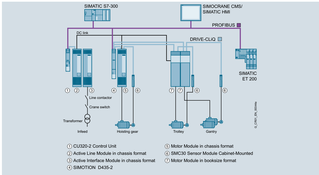
Bridge crane topology with chassis and booksize formats
