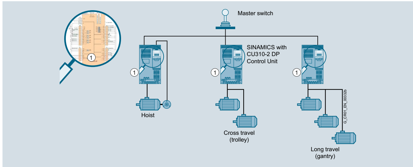
Topology with onboard I/O
