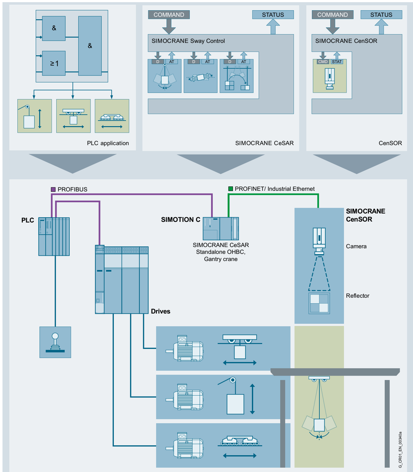
Configuration SIMOCRANE CeSAR standalone OHBC, gantry crane
