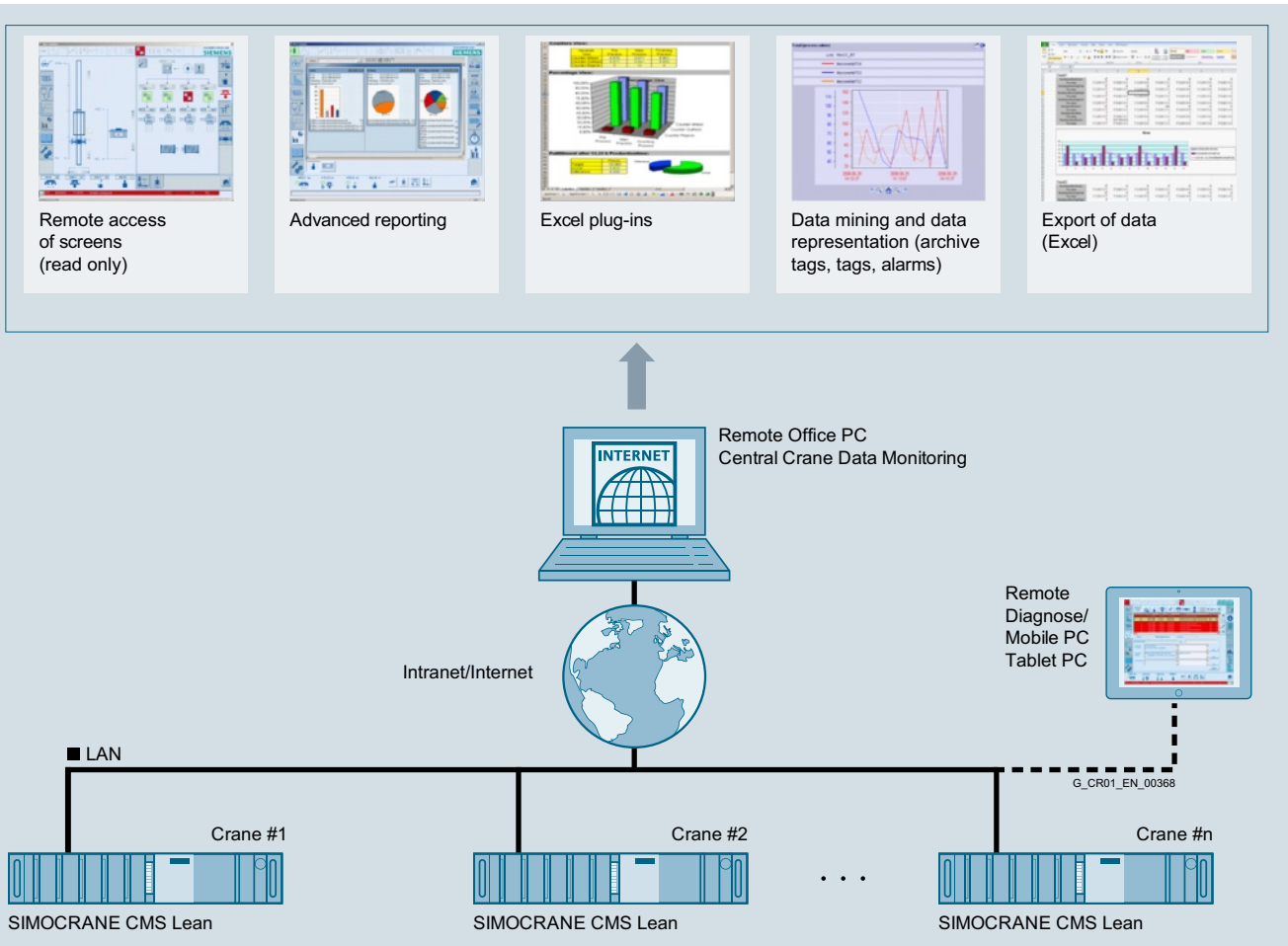
Overview of CMS Central Crane DataMonitor
