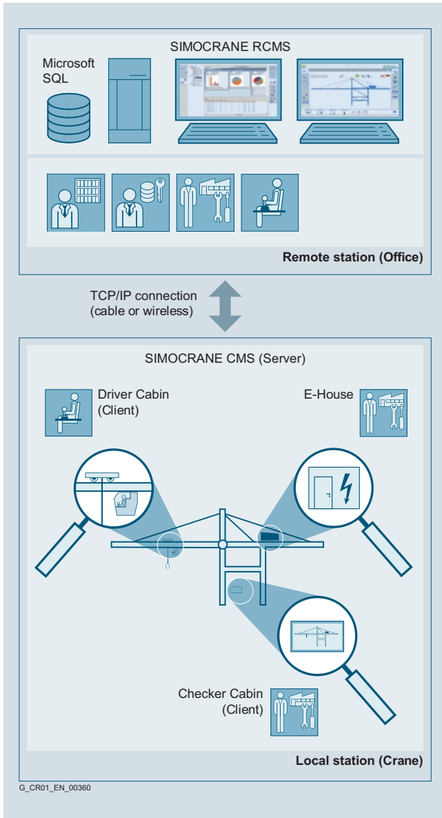
Example for solution configuration for an STS crane using SIMOCRANE CMS and RCMS
