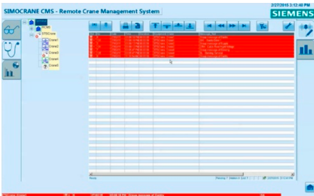
RCMS – message list for all cranes in the terminal
