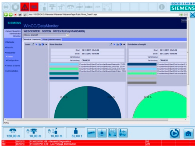
Graphical data representation in DataMonitor
