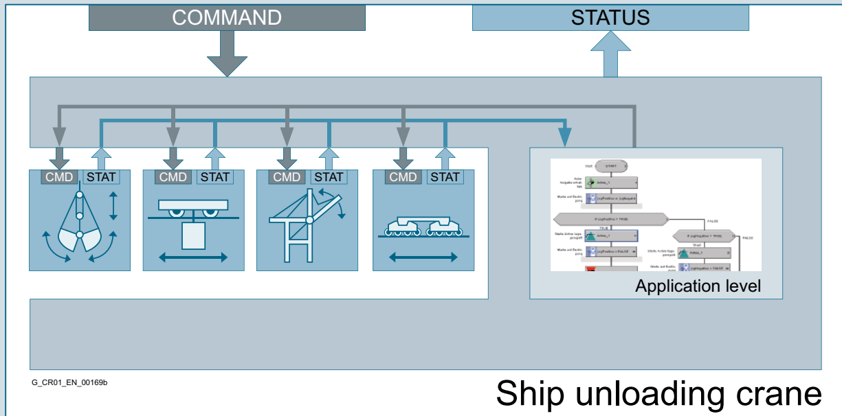
Function blocks for ship unloading crane
