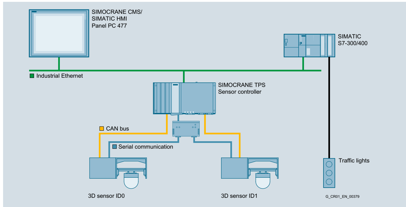
TPS topology for STS crane
