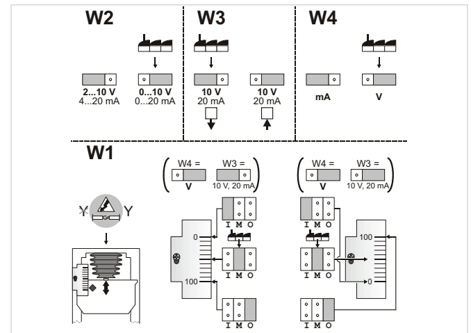
Fig. 2 Effects of jumper plugs W1, W2, W3, W4
