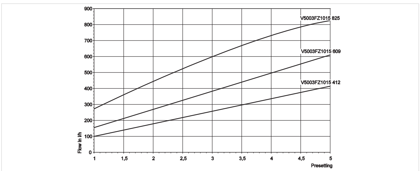
Fig. 4 Presetting Diagram Kombi VX V5003FY10
