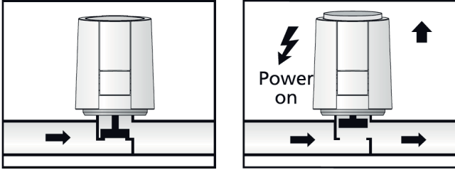
Fig. 1 Extrusion of the function display when valve opens
