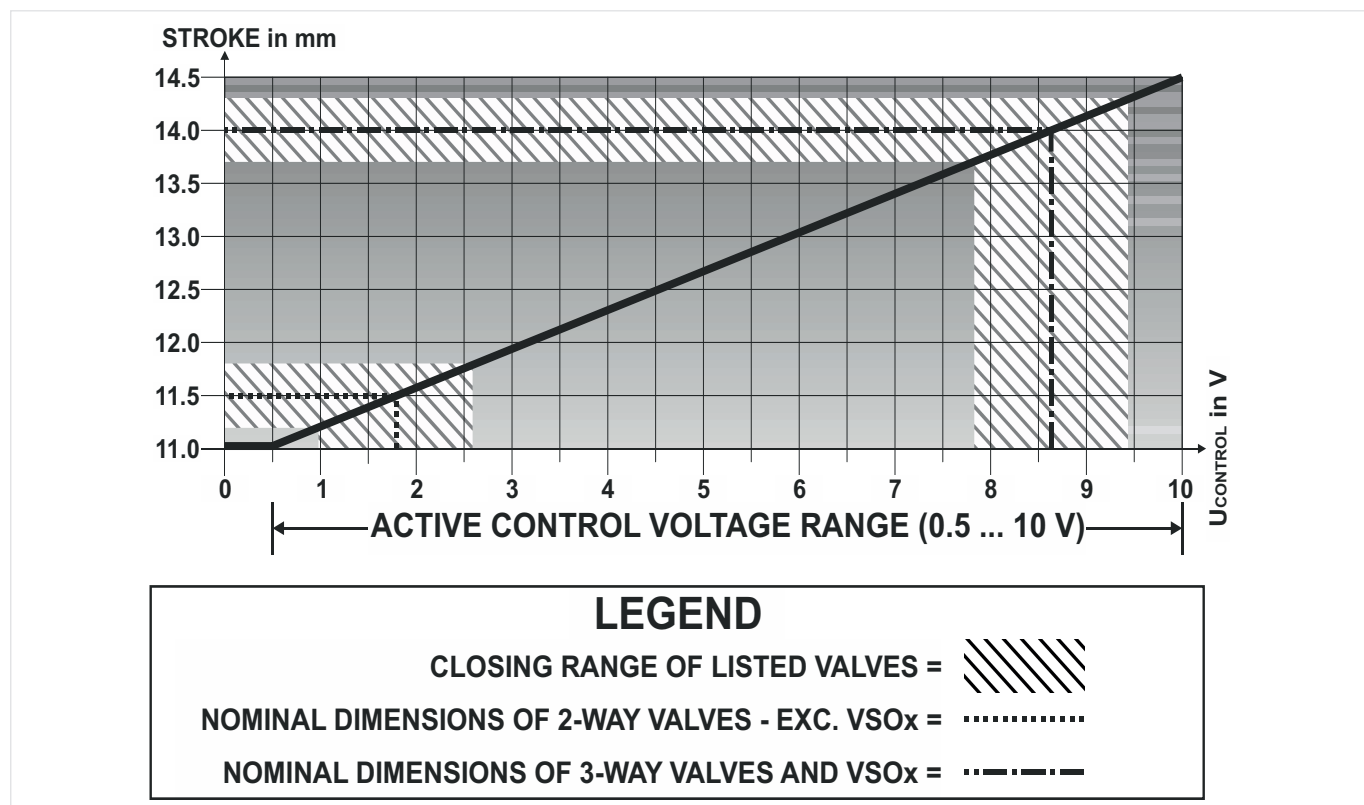
Fig. 8 Characteristic (stroke vs. voltage)
