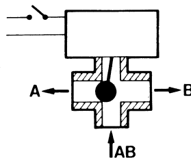
V8044C (24 V, 50 Hz)
