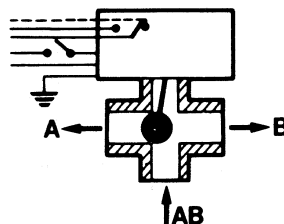
V4044F (220 Vac, 50 Hz)
