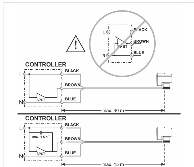
Fig. 1 Electrical wiring M5410L1001
