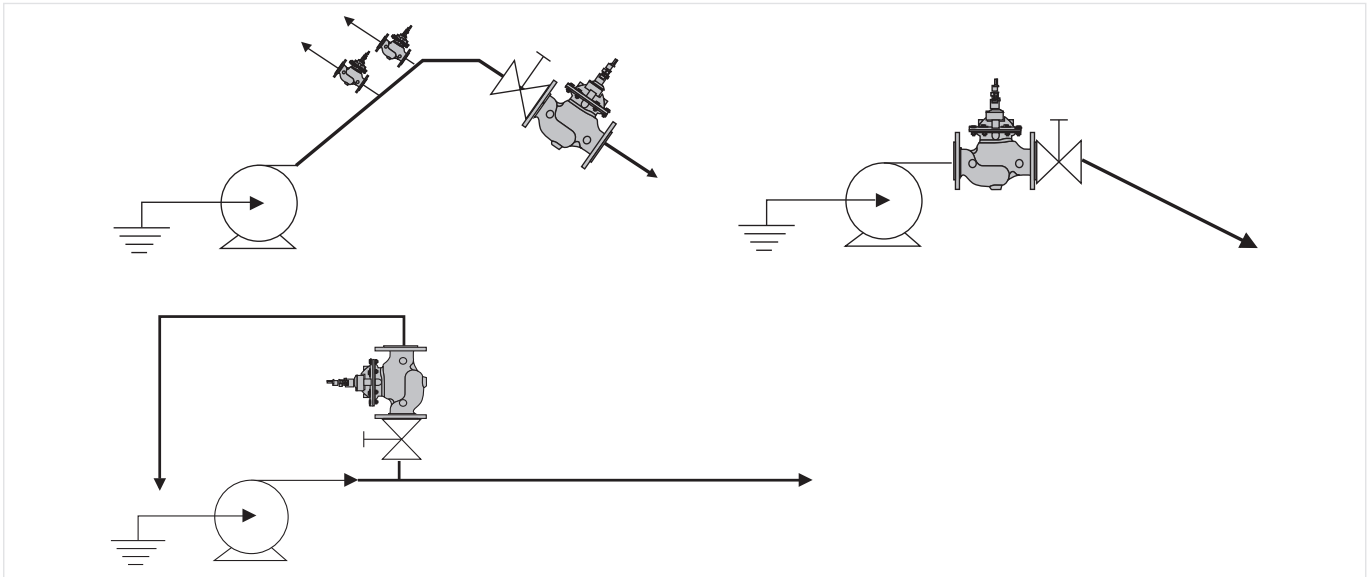
Fig. 1 Standard installation example for the pressure sustaining valve
