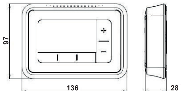
T4, T4M Thermostat
