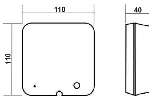
Receiver box
