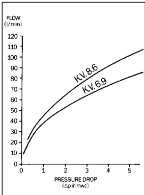
Fig. 2. Flow Characteristics
