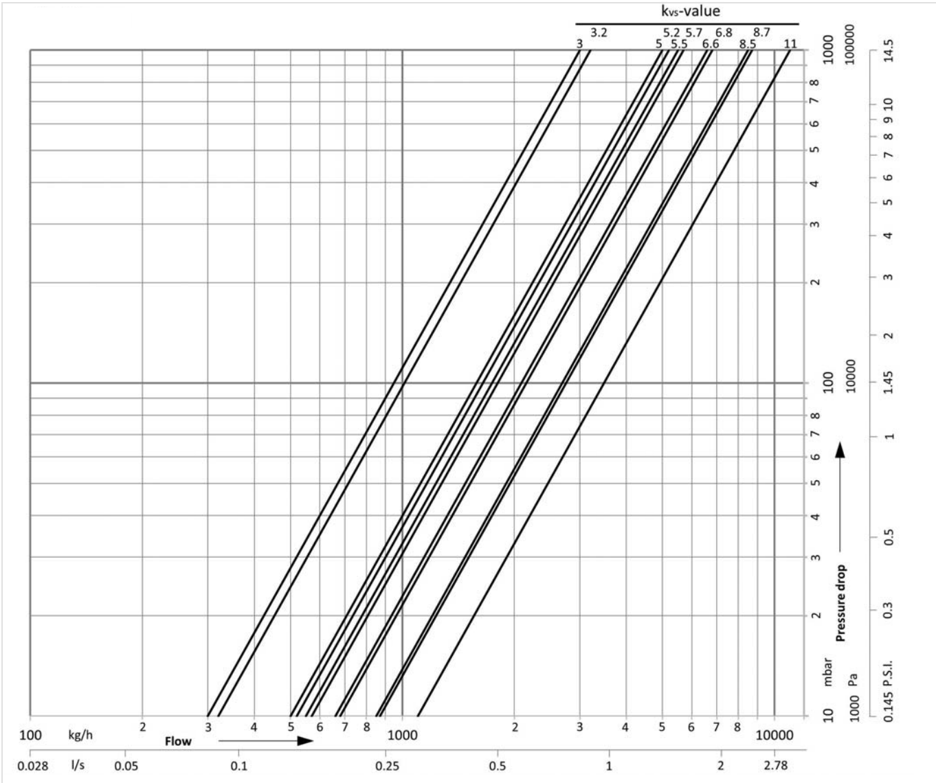
Fig. 7 Valve pressure loss characteristic
