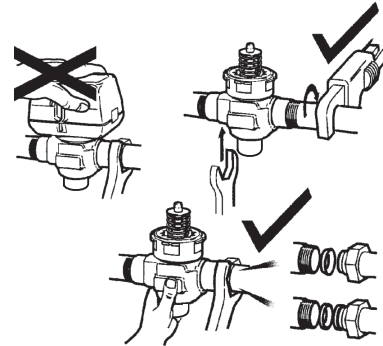
Fig. 2. Plumbing of the VC valve.
