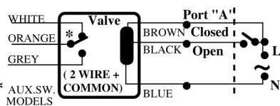
Fig. 7. Wiring color code for cable models for SPST controller. (Series 40 & 80)
