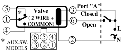
Fig. 6. Wire configuration for MOLEX™ models for SPST controller. (Series 40 & 80)
