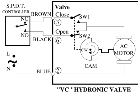
Fig. 8. Actuator wiring for SPDT controller
