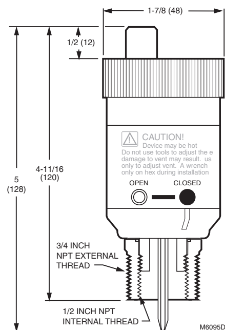
Fig. 1. EA79 dimensions in in. [mm].
