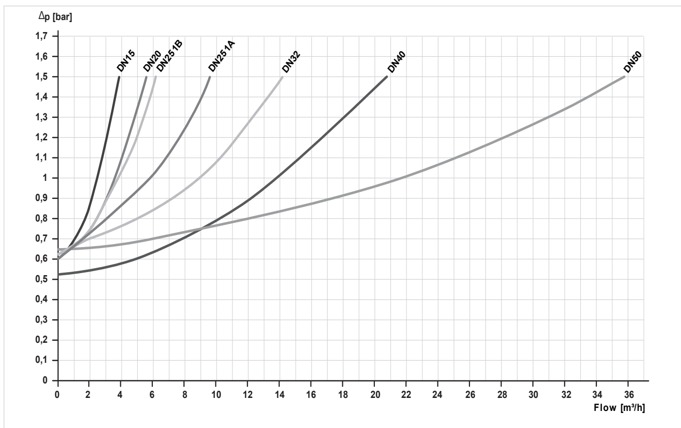
Fig. 1 Pressure drop within the valve in dependency of the flow rate and the used connection size
