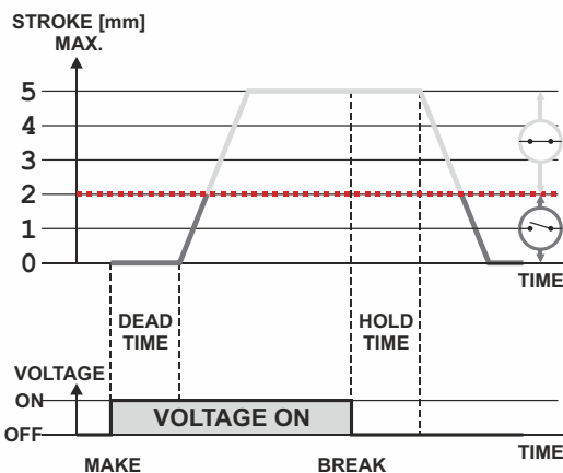
Fig. 4 Opening / closing time of N.C. versions with auxiliary switch
