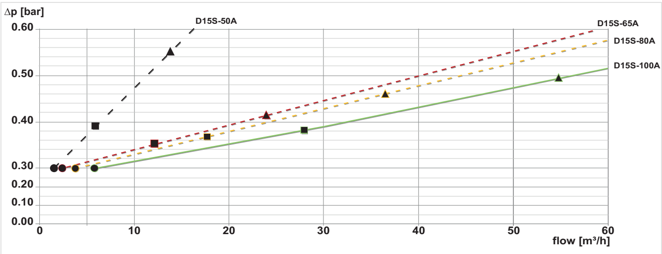
Fig. 2 Pressure drop within the valve in dependency of the flow rate and the used connection size (Sizes 50-100) Pressure setting: P1: 8 bar, P2: 3 bar
