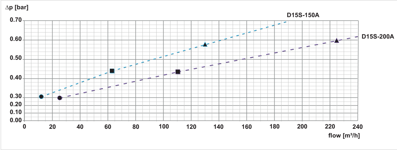
Fig. 3 Pressure drop within the valve in dependency of the flow rate and the used connection size (Sizes 150-200) Pressure setting: P1: 8 bar, P2: 3 bar
