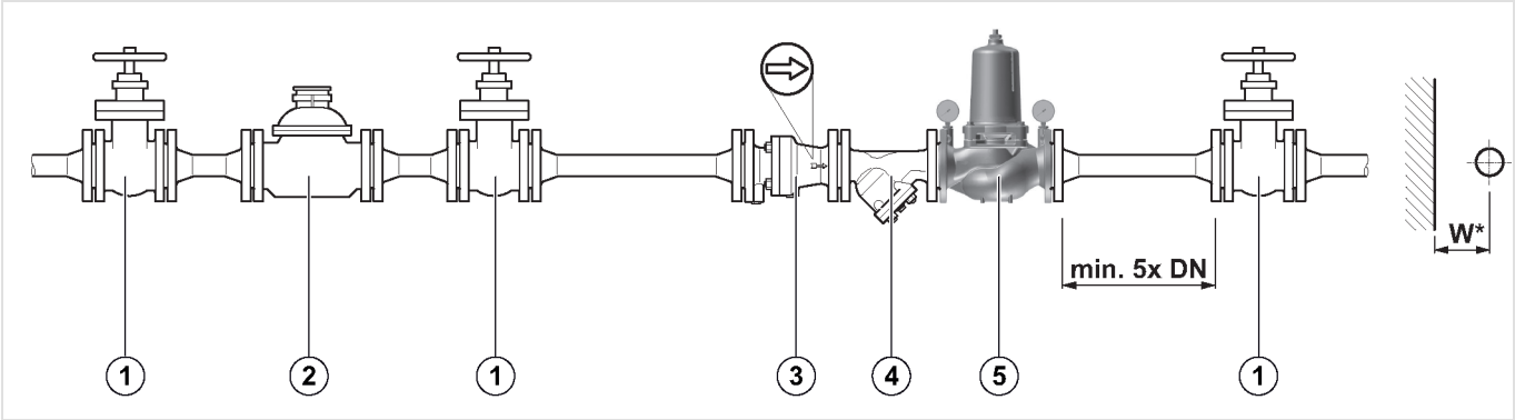
Fig. 1 Standard installation example for the pressure reducing valve
