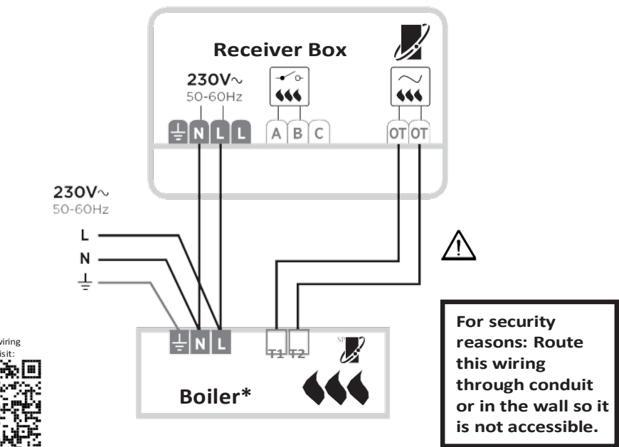
D) OpenTherm boiler
