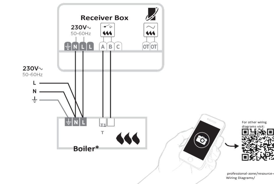
C) Combi boiler
