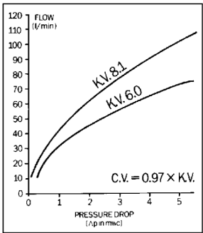
Fig. 2. Flow Characteristics.
