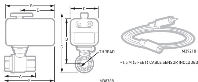
Fig. 1. Dimension diagram.
