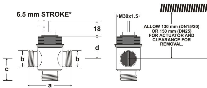
Fig. 2. VXE... (3-way), dimensions
