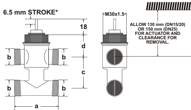
Fig. 3. VYE... (3-way with bypass), dimensions
