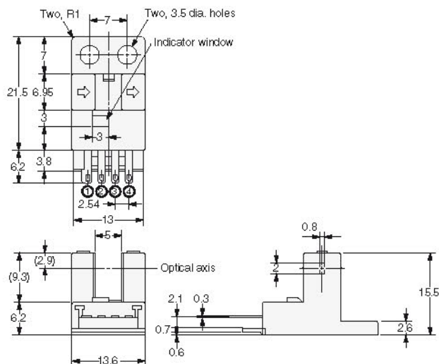
Terminal Arrangement
