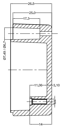
SECTION B-B
