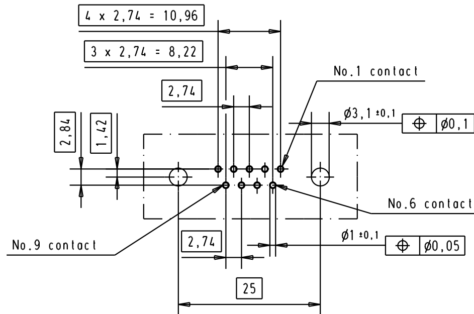
Printed board layout component side
