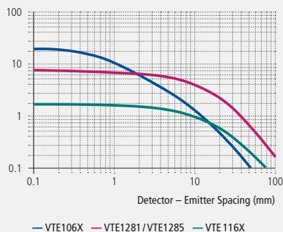
On Axis Relative Irradiance
