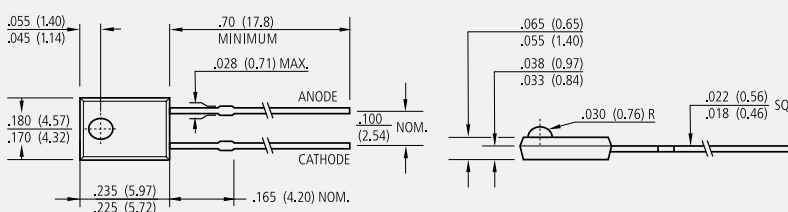
Housing / Package Drawing – VTE7172
