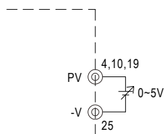
Fig. 3.1 Add on 0~5V external voltage
