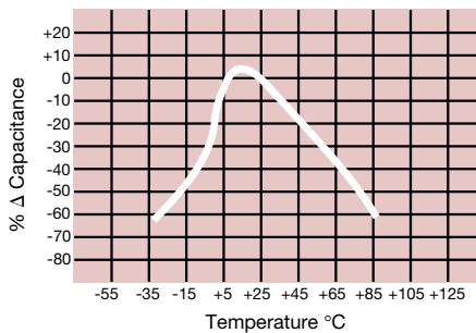
Temperature Coefficient
