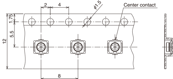
U.FL-R-SMT-1(60) : 8mm pitch
