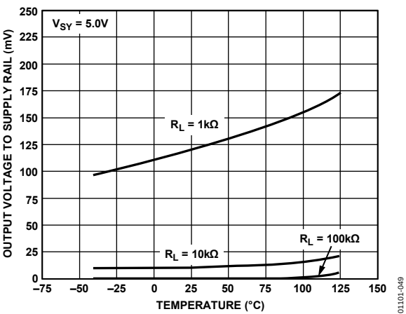
Figure 49. Output Voltage to Supply Rail vs. Temperature
