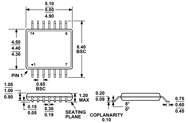
Figure 74. 14-Lead Thin Shrink Small Outline Package [TSSOP] (RU-14) Dimensions shown in millimeters
