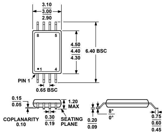
Figure 72. 8-Lead Thin Shrink Small Outline Package [TSSOP] (RU-8) Dimensions shown in millimeters
