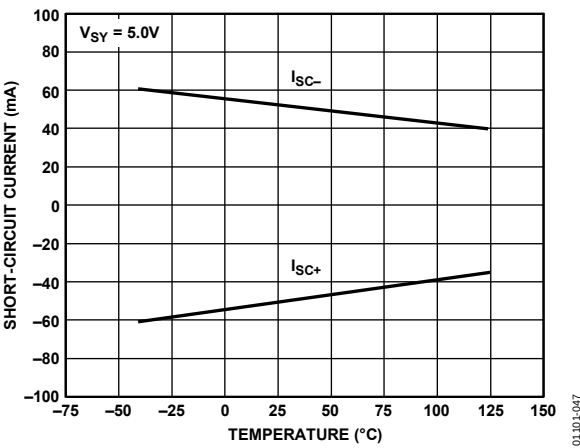
Figure 47. Output Short-Circuit Current vs. Temperature
