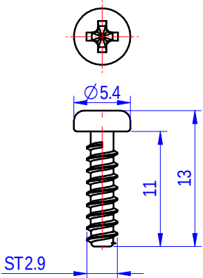
3、DGBSC-PG01-00Z-screws
