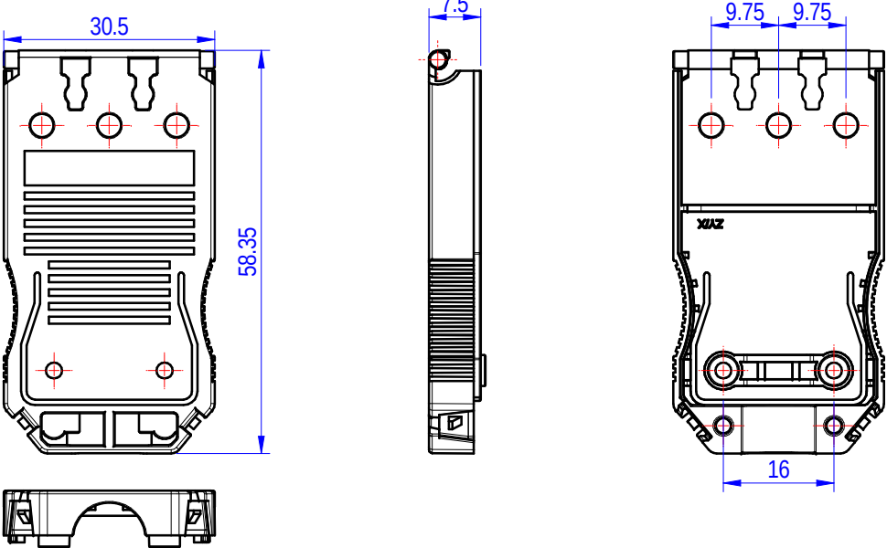
2、DGBSC-PG01M&F/4-03P-00ZH-bottom
