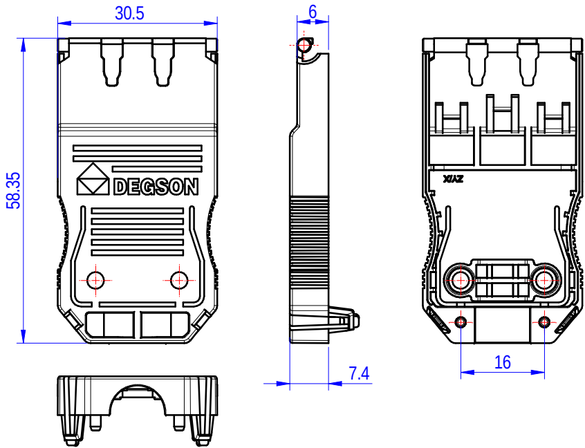
1、DGBSC-PG01M&F/4-03P-00ZH-top cover
