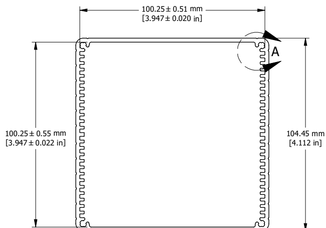
EXTRUSION
