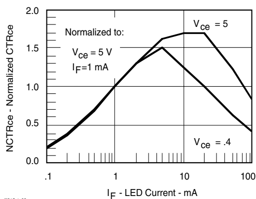
Figure 8. Normalized Non-Saturated and Saturated CTR_{CE} vs. LED Current
