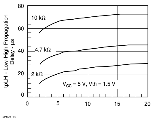
Figure 13. Low to High Propagation Delay vs. LED Current and Load Resistor
