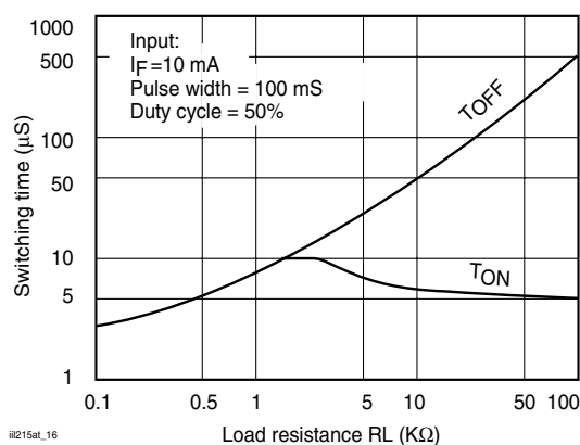
Figure 16. Typical Switching Times vs. Load Resistance
