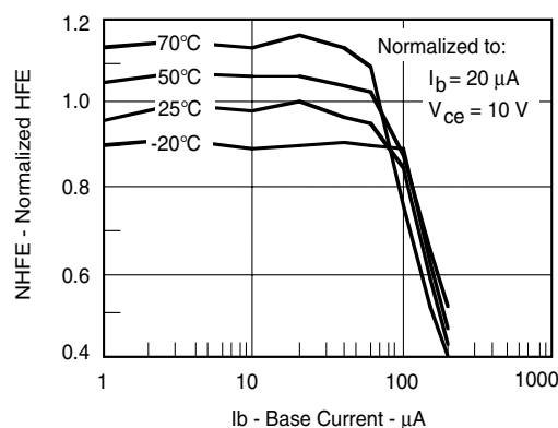
Figure 14. Normalized Non-saturated HFE vs. Base Current and Temperature
