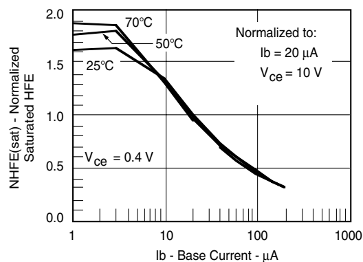
Figure 7. Normalized Saturated HFE vs. Base Current and Temperature
