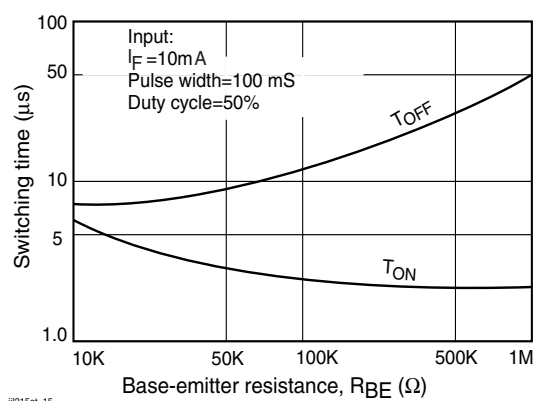
Figure 15. Typical Switching Characteristics vs. Base Resistance (Saturated Operation)
