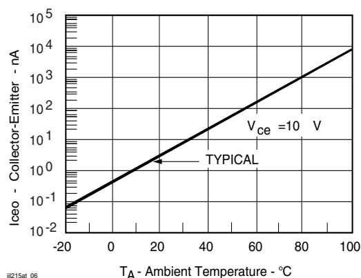
Figure 6. Collector-Emitter Leakage Current vs. Temp.
