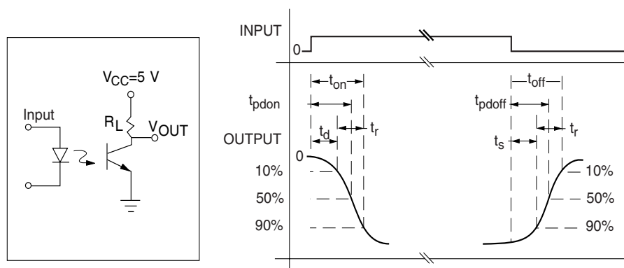
Figure 17. Switching Test Circuit
