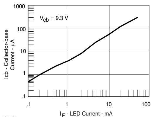
Figure 5. Collector-Base Photocurrent vs. LED Current
