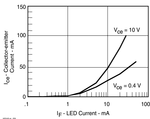
Figure 3. Collector-Emitter Current vs. LED Current
