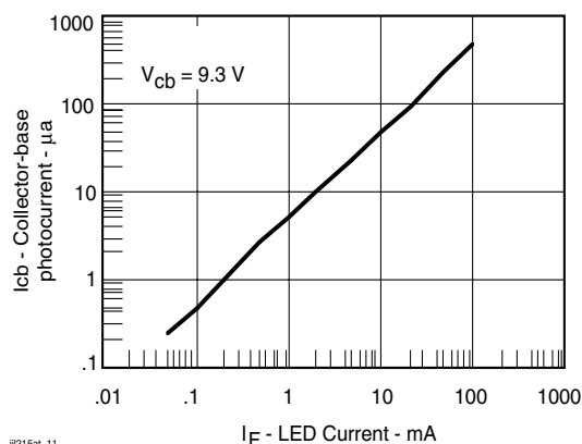
Figure 11. Collector-Base Photocurrent vs. LED Current
