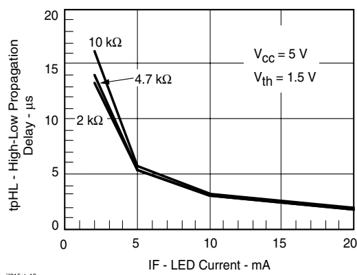
Figure 12. High to Low Propagation Delay vs. LED Current and Load Resistor
