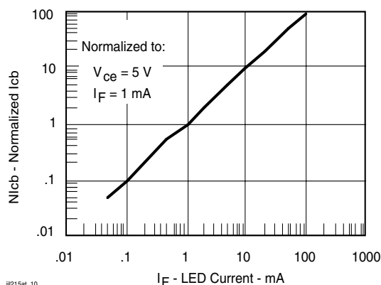
Figure 10. Normalized Collector-Base Photocurrent vs. LED Current
