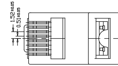
CONTACT 2 PRONGS FOR STRANDED WIRE
