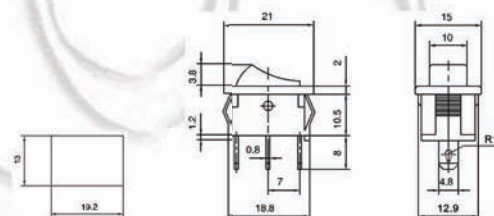
RSM102 RSM102A ON-ON RSM103 RSM103A ON-OFF-ON RSM112 RSM112A ON-(ON) SPDT 3P
