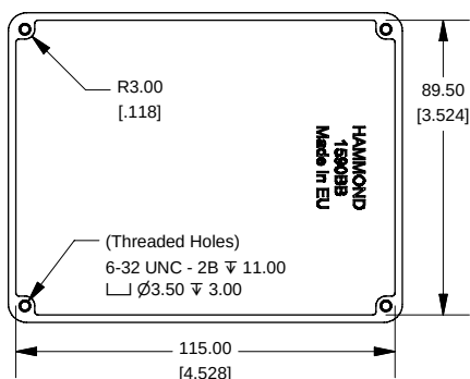
Top View Looking Inside Box
