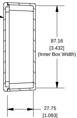
SECTION A-A End View of Assembly
