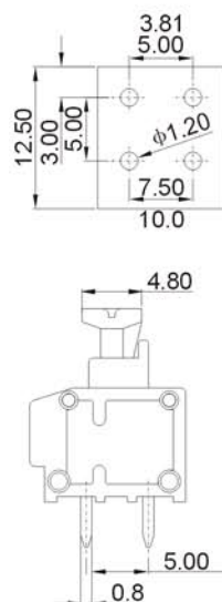
PCB LAYOUT
