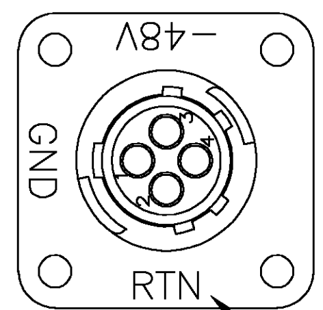
DETAIL A -5 ONLY RTN, GND AND -48V MARKED WITH WHITE INK, .118 MAX.
