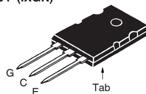
TO-264 (IXGK)
