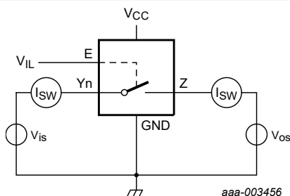
Fig. 9. Test circuit for measuring OFF-state leakage current
