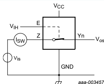
Fig. 10. Test circuit for measuring ON-state leakage current
