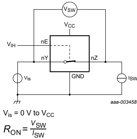
Fig. 7. Test circuit for measuring R_{ON}
