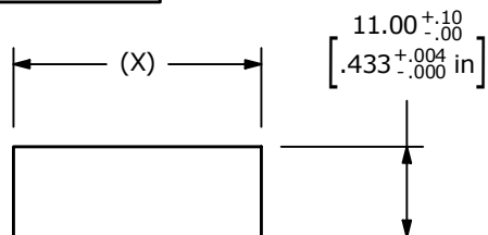
PANEL CUTOUT
