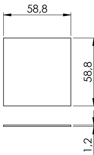
Rear panel (1:2)
