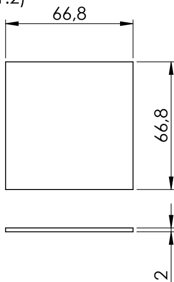
Filter (1:2)
