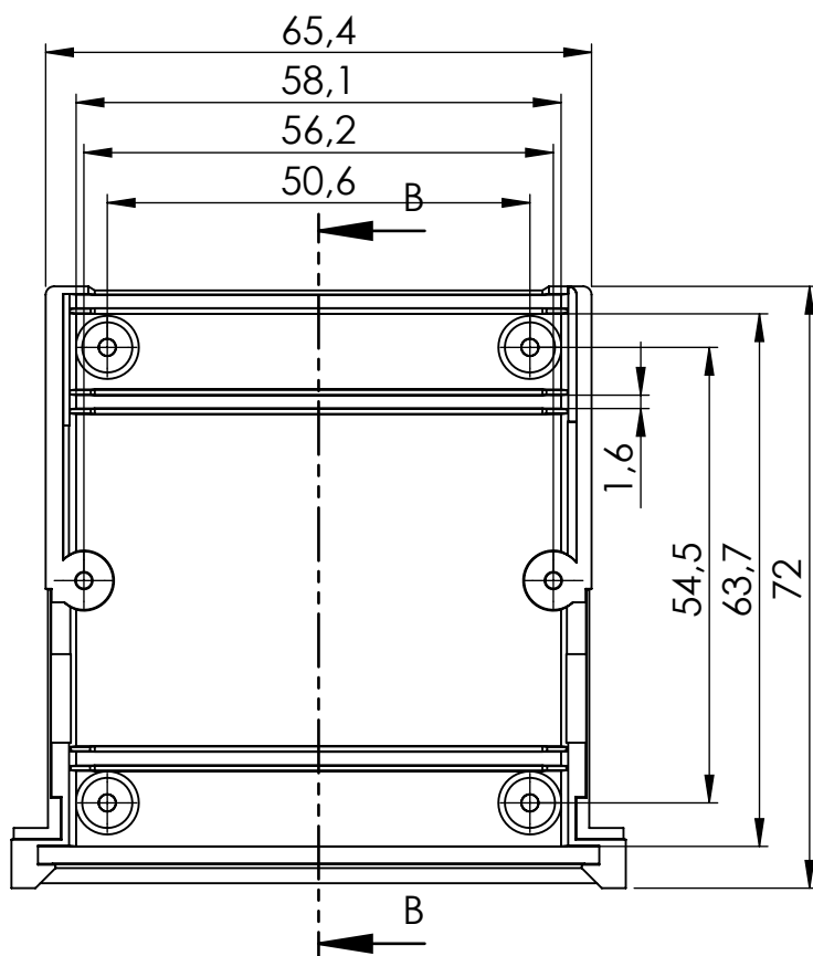
Rear panel (1:2)
