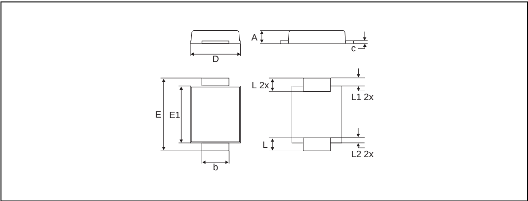
Figure 23. SMAflat dimension definitions
