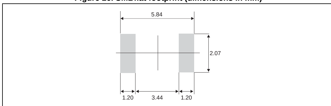
Figure 26. SMBflat footprint (dimensions in mm)
