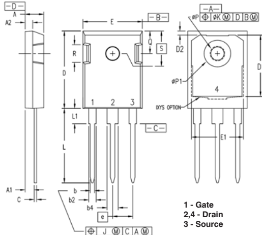
TO-247 Outline
